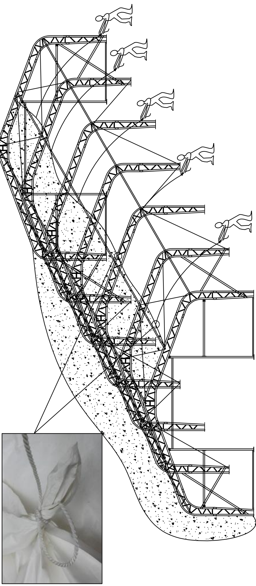
Figure 8 Pull the Roof Cover over the frame evenly
